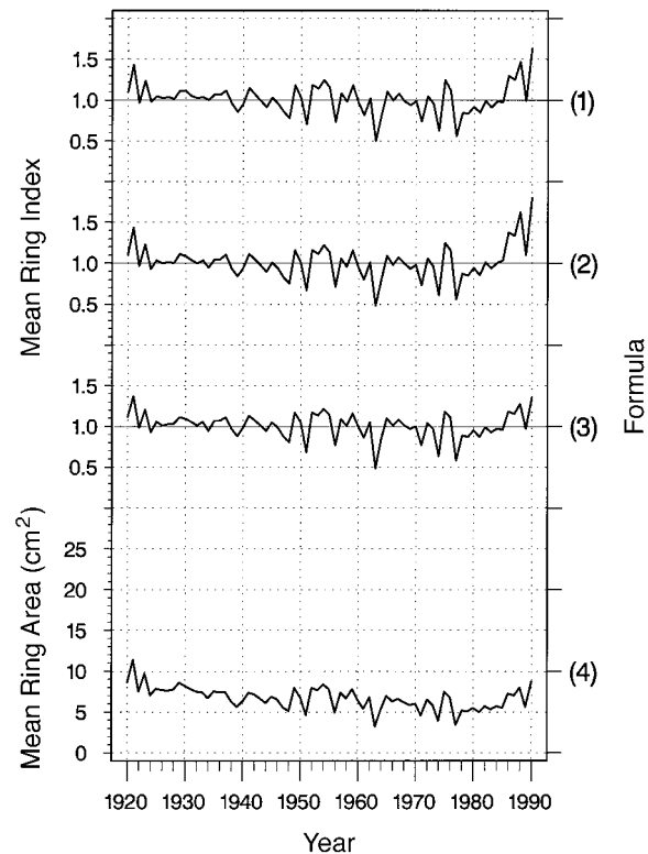
FIG. 5. The same as Fig. 4, but for pines with 1990 dbh < 50 cm (SMALL PINES).
