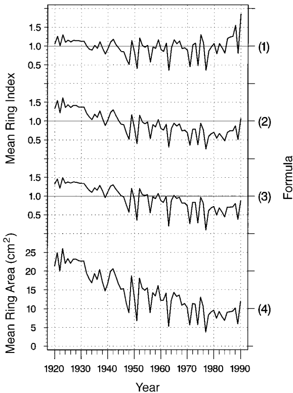
FIG. 4. Tree-ring chronologies from 1920 to 1990 based on tree-ring samples of pines with 1990 dbh > 50 cm (LARGE PINES). The four methods [(1) ARSTAN, (2) Fritts, (3) Biondi, and (4) Phipps] used to compute the chronologies are detailed in Materials and Methods: Tree-ring data .
